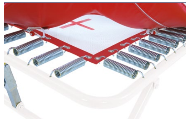
34 galvanized springs connected to the PVC bed
