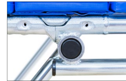
New frame design with laser cut parts giving greater potential for safety
